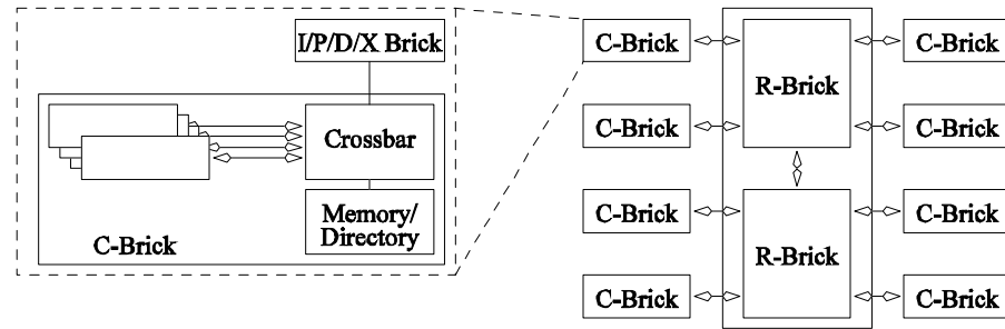
32 Processor Configuration
