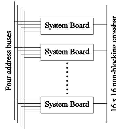
Starfire Ultra 1000 (up to 64 processors)
