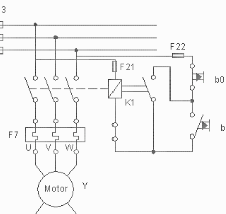
Diagrama Multifilar
