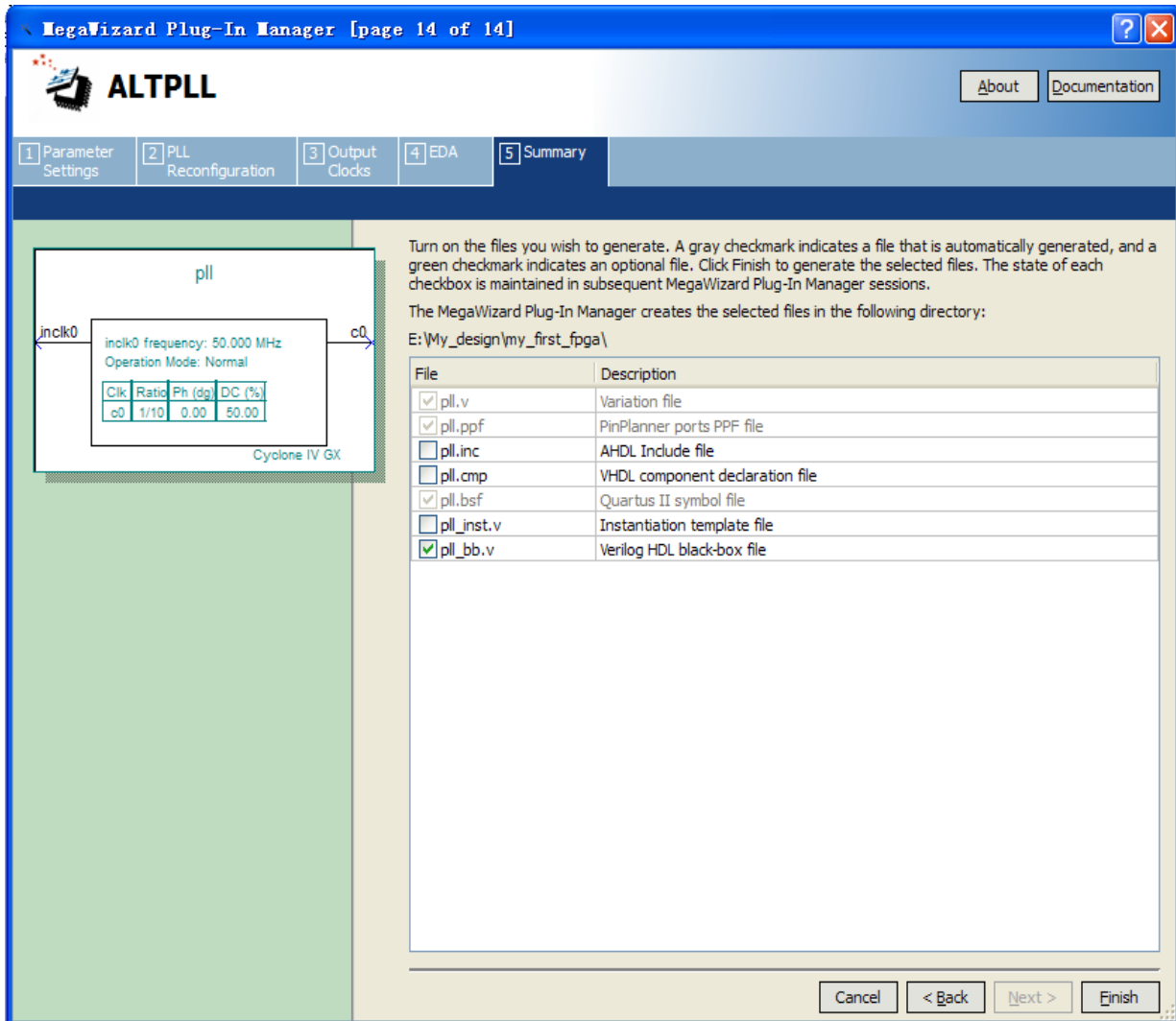
Figure 3-13 Wizard-Created Files
