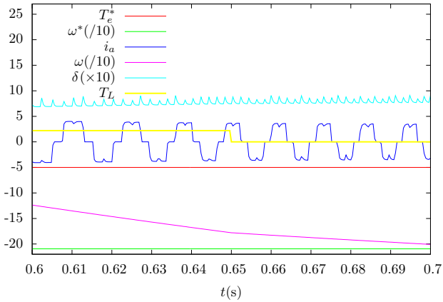
Fig. 10. Detail of BLDC motor operation, showing PWM duty cycle.
