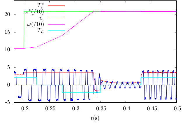
Fig. 8. BLDC motor with proposed SMC using tanh function as analog sign function.
