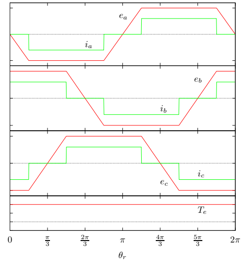
Fig. 1. Brushless DC motor ideal electromagnetic torque generation.
