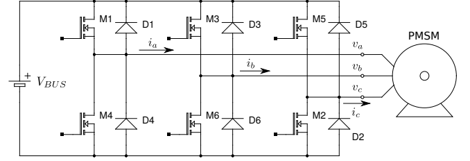
Fig. 3. Three-phase inverter bridge and PMSM machine.
