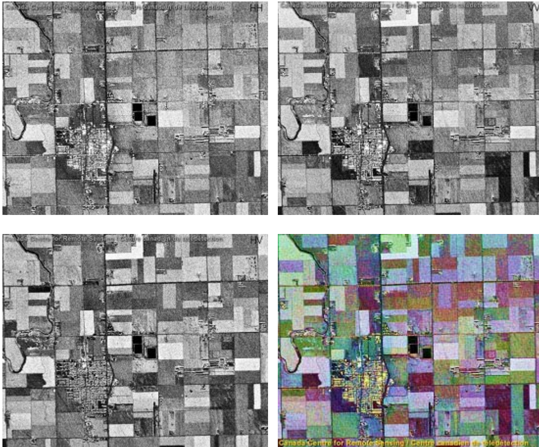
Illustration of how different polarizations (HH, WV, HV & colour composite) bring out different features in an agricultural scene
