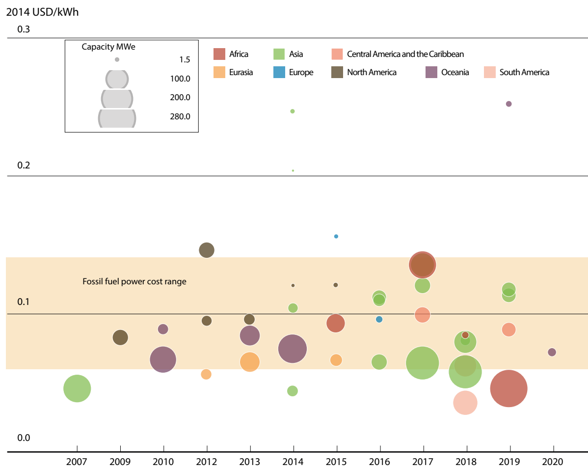
FIGURE 9.5: THE LEVELISED COST OF ELECTRICITY OF GEOTHERMAL POWER PROJECTS BY REGION AND SIZE
