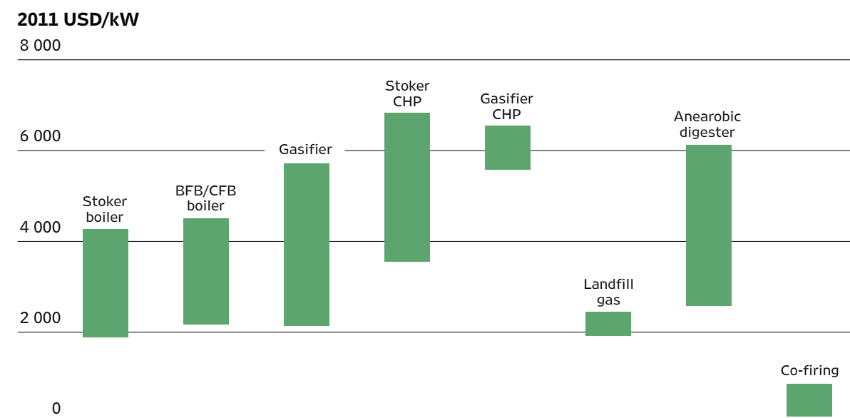
FIGURE 8.4: TYPICAL TOTAL INSTALLED CAPITAL COSTS OF BIOMASS-FIRED ELECTRICITY GENERATION TECHNOLOGIES IN OECD COUNTRIES
