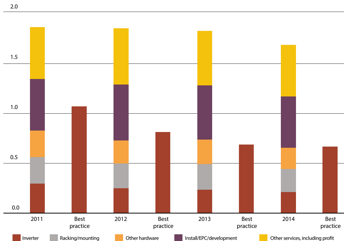
FIGURE 5.6: GLOBAL AVERAGE BALANCE OF SYSTEM COST BREAKDOWN AND GLOBAL BEST PRACTICE AND BoS COSTS IN ITALY BY PROJECT SIZE, 2011-2014
