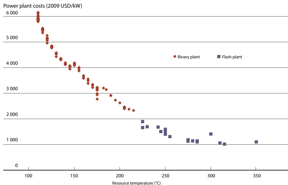
FIGURE 9.3: INDICATIVE POWER PLANT ONLY COSTS FOR GEOTHERMAL PROJECTS BY RESERVOIR TEMPERATURE
