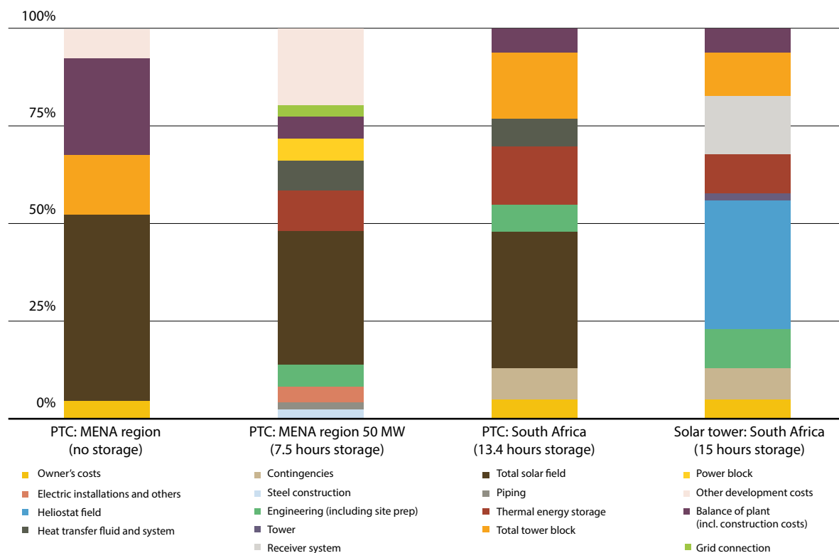
FIGURE 6.3: INDICATIVE BREAKDOWN OF CSP INSTALLED COSTS BY TECHNOLOGY AND AMOUNT OF STORAGE
