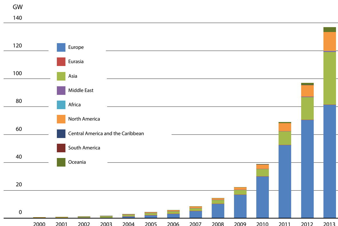
FIGURE 5.1: GLOBAL CUMULATIVE INSTALLED SOLAR PHOTOVOLTAIC CAPACITY, 2000-2014
