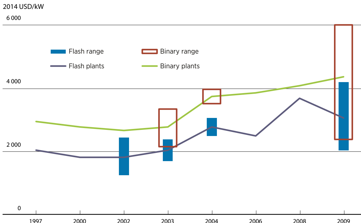
FIGURE 9.1: TOTAL INSTALLED COSTS FOR GEOTHERMAL POWER STATIONS, 1997 TO 2009
