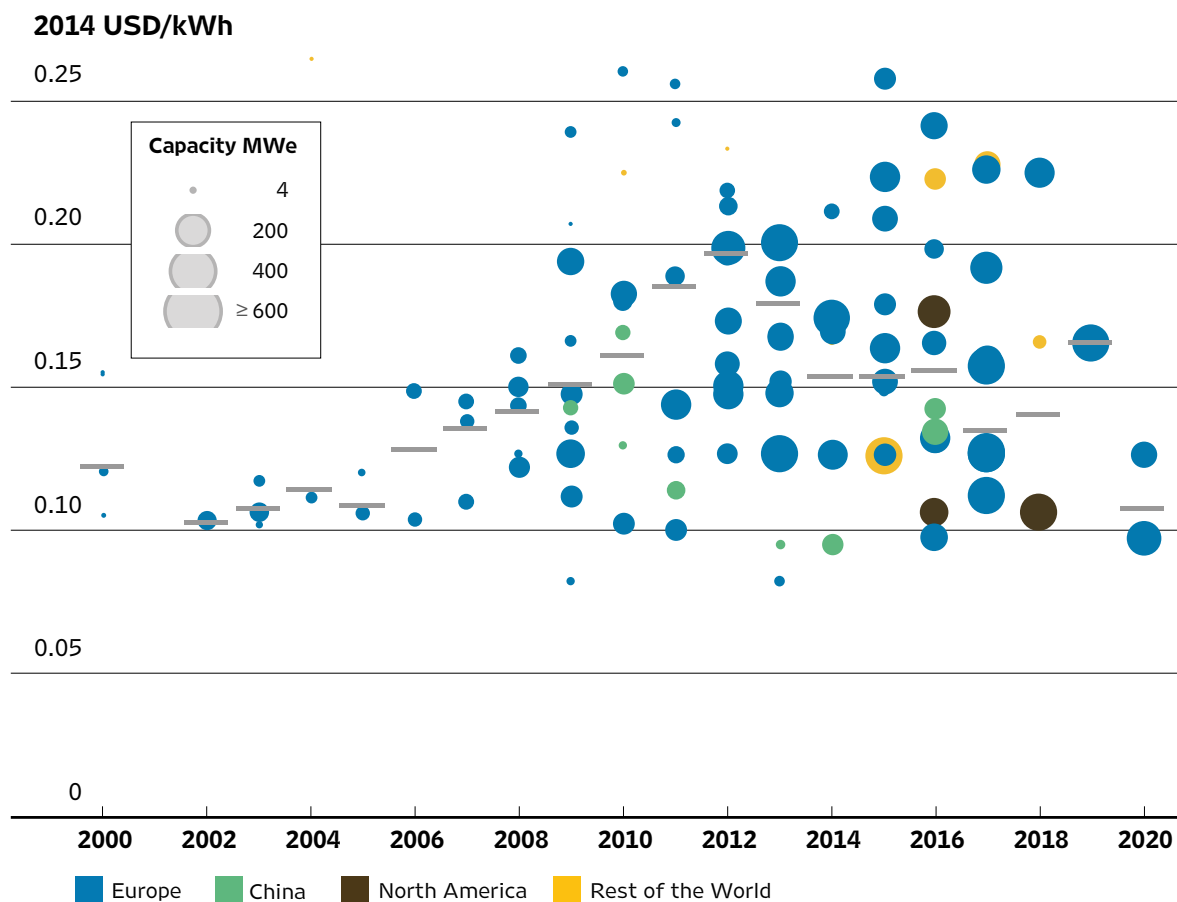
FIGURE 4.19: THE LCOE AND WEIGHTED AVERAGES OF COMMISSIONED AND PROPOSED OFFSHORE WIND PROJECTS, 2000 TO 2020
