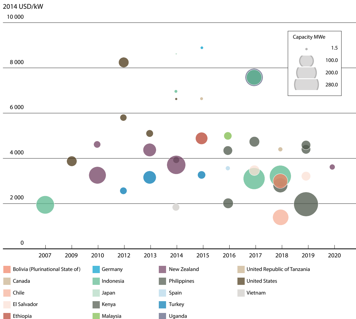
FIGURE 9.2: INSTALLED CAPITAL COSTS FOR GEOTHERMAL POWER PROJECTS, 2007 TO 2020
