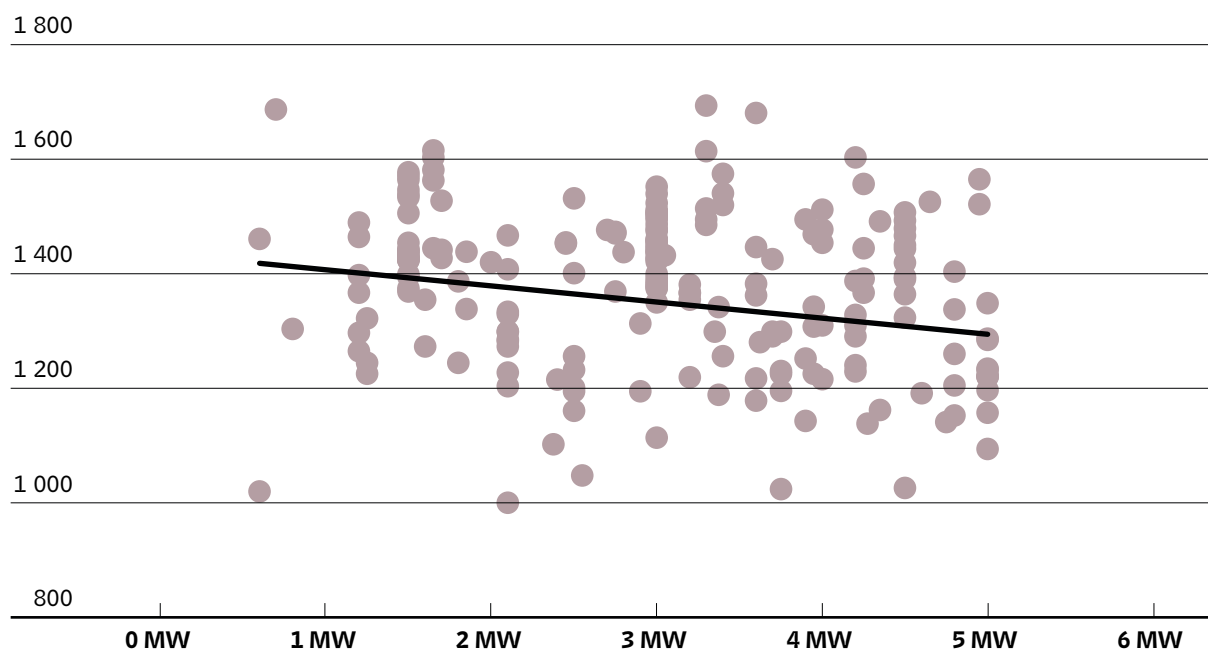
FIGURE 4.5: TOTAL INSTALLED COSTS OF COMMISSIONED SMALL WIND FARMS IN INDIA (<5 MW), 2000-2013 2014 USD/kW
