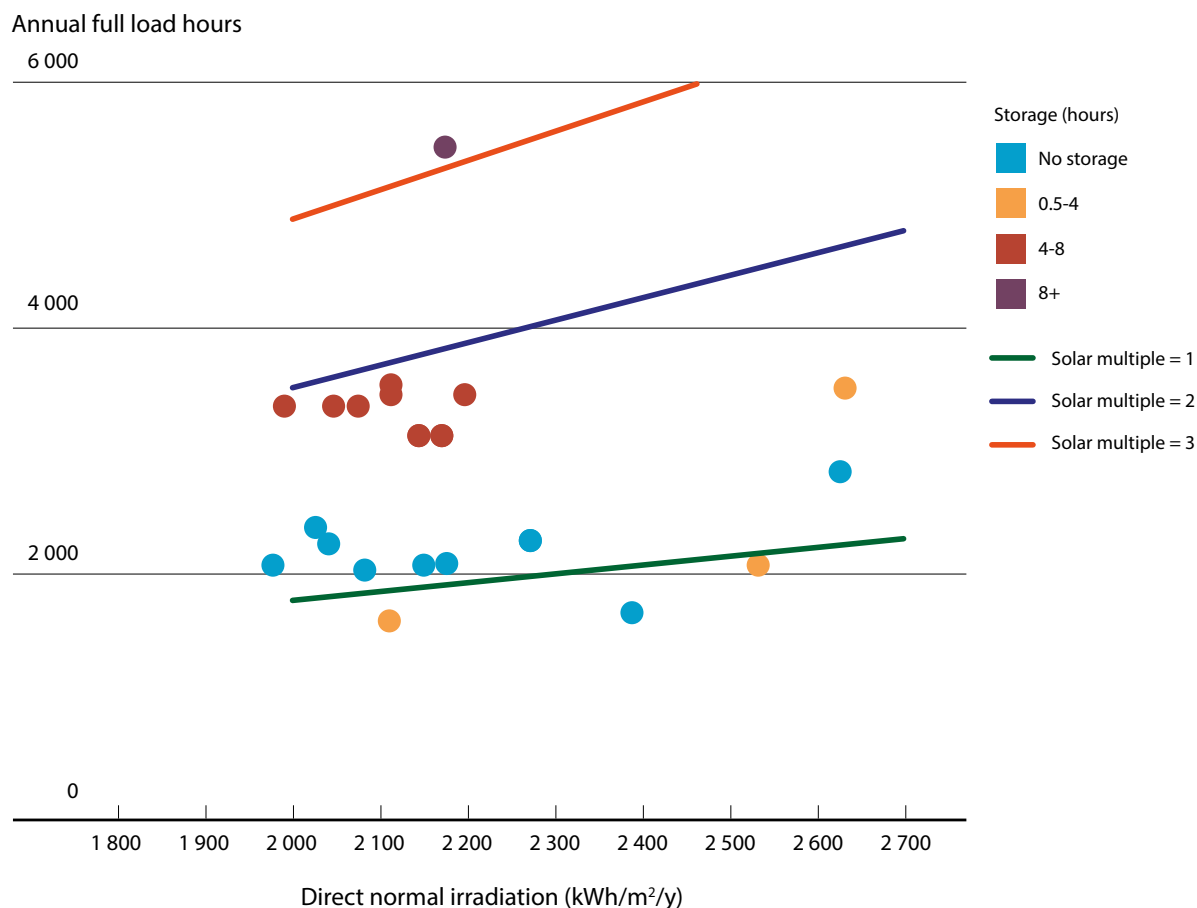
FIGURE 6.5: FULL LOAD HOURS FOR CSP PROJECTS AS A FUNCTION OF DIRECT NORMAL IRRADIANCE AND STORAGE CAPACITY
