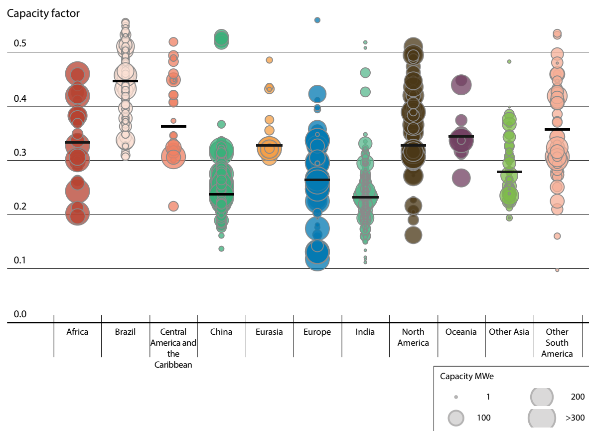
FIGURE 4.12: CAPACITY FACTORS BY PROJECT AND WEIGHTED AVERAGES FOR COMMISSIONED AND PROPOSED WIND FARMS, 2010-2014
