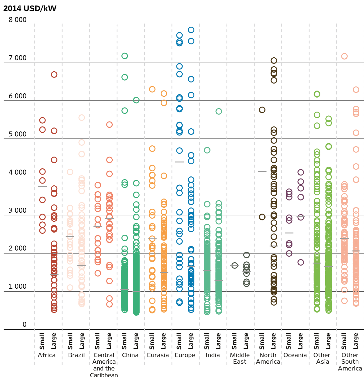
FIGURE 7.3: TOTAL INSTALLED COST RANGES AND CAPACITY WEIGHTED AVERAGES FOR COMMISSIONED OR PROPOSED SMALL AND LARGE HYDROPOWER PROJECTS BY COUNTRY/REGION
