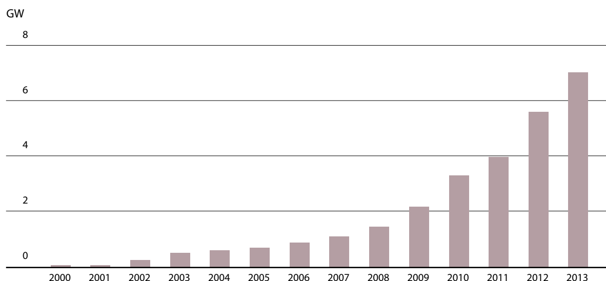
FIGURE 4.8: CUMULATIVE OFFSHORE WIND INSTALLED CAPACITY AT THE END OF 2013
