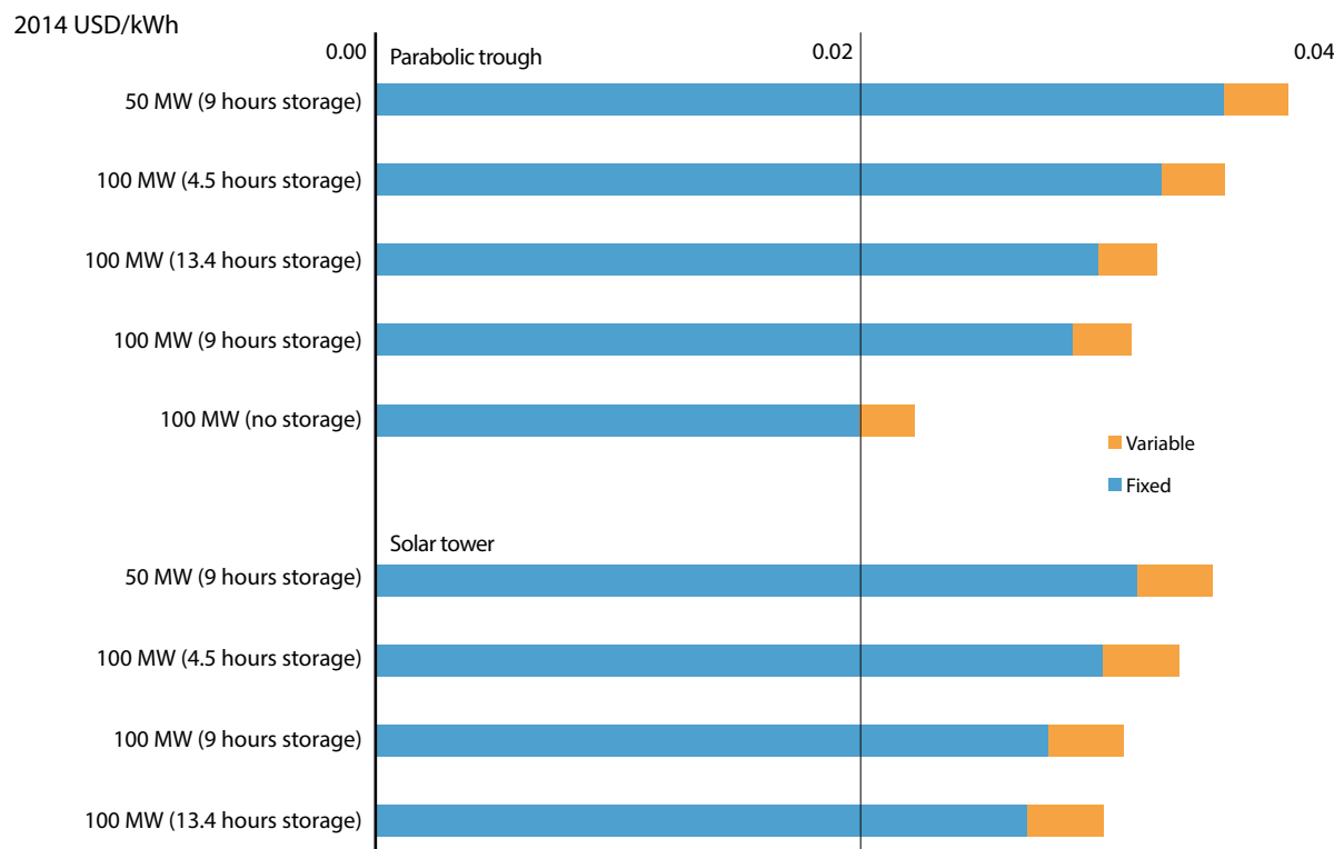
FIGURE 6.4: OPERATIONS AND MAINTENANCE COSTS FOR PARABOLIC TROUGH AND SOLAR TOWER CSP PLANTS
