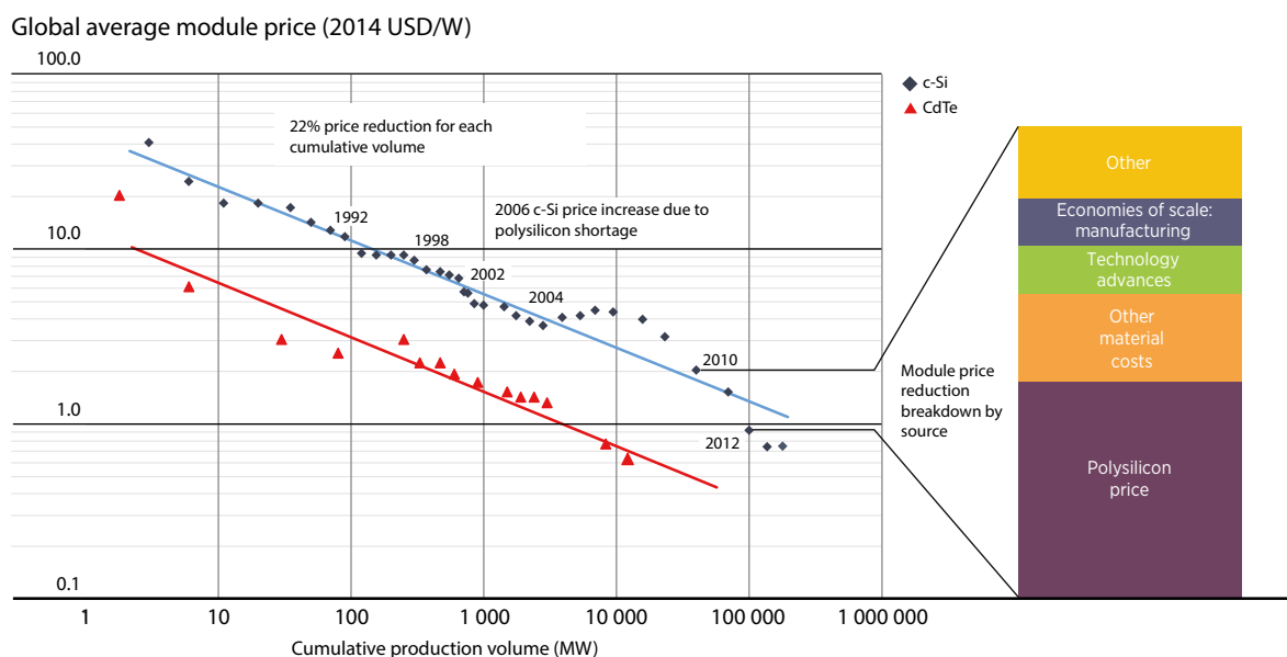
FIGURE 5.4: SOLAR PV CRYSTALLINE SILICON AND THIN-FILM MODULE COST LEARNING CURVE
