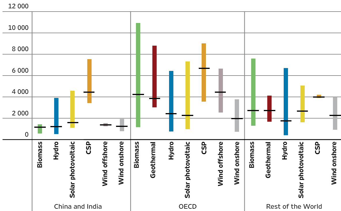
FIGURE 2.8: TYPICAL RANGES AND WEIGHTED AVERAGES FOR THE TOTAL INSTALLED COSTS OF UTILITY-SCALE RENEWABLE POWER GENERATION TECHNOLOGIES BY REGION, 2013/2014
