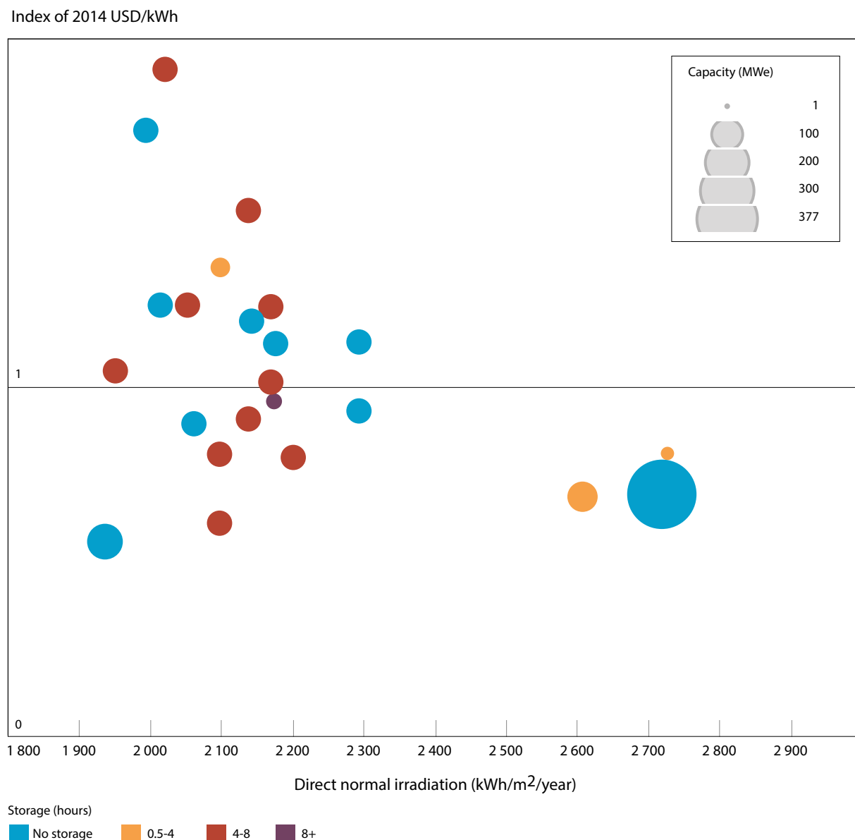
FIGURE 6.7: INDEX OF THE LEVELISED COST OF ELECTRICITY AS A FUNCTION OF DIRECT NORMAL IRRADIANCE FOR A RANGE OF CSP PROJECTS
