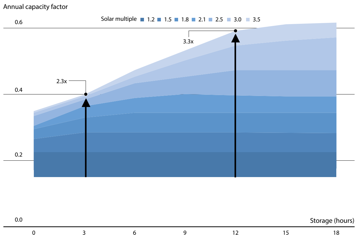
FIGURE 6.6: CAPACITY FACTOR FOR A 100 MW PTC PLANT AS A FUNCTION OF SOLAR MULTIPLE AND THERMAL ENERGY STORAGE
