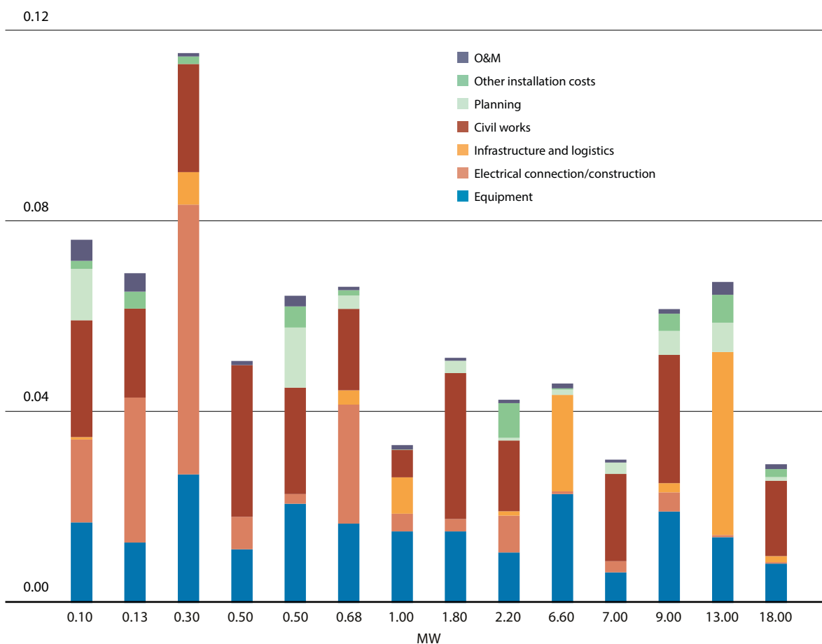
FIGURE 7.8: THE LEVELISED COST OF ELECTRICITY BREAKDOWN BY COST COMPONENT FOR 14 SMALL HYDROPOWER PROJECTS IN DEVELOPING COUNTRIES
