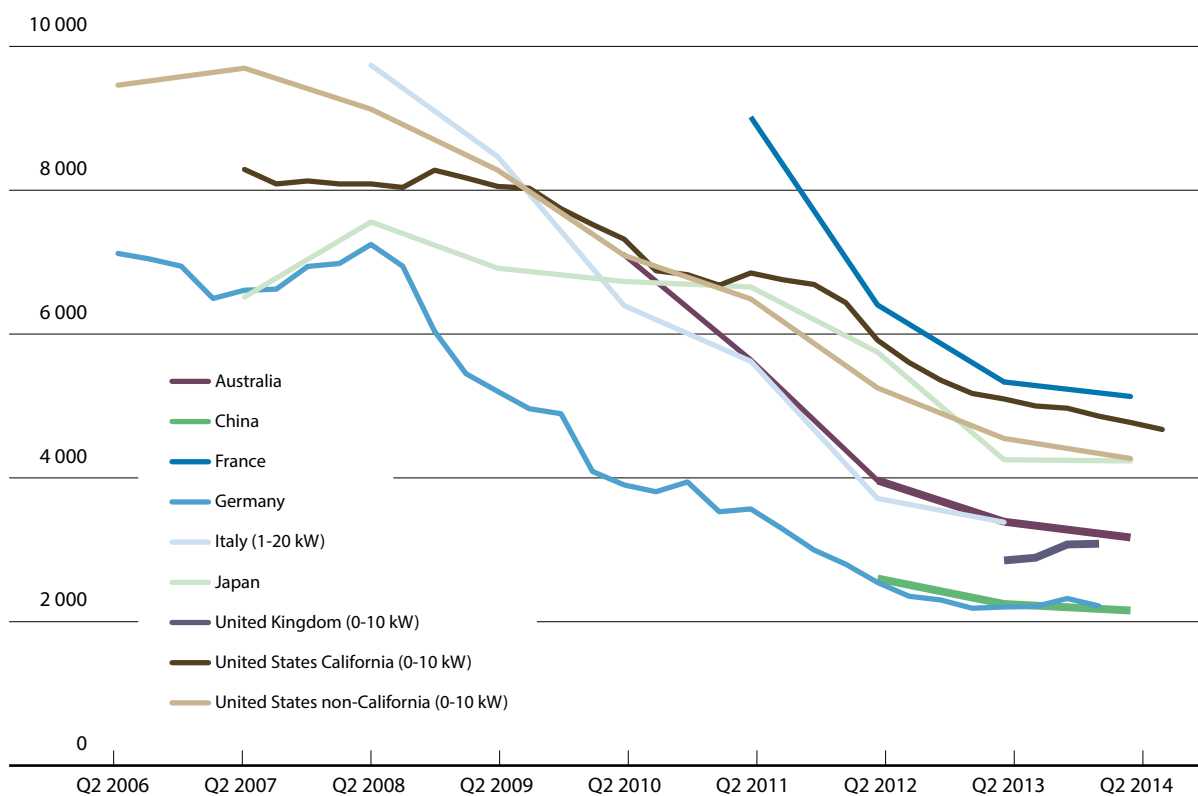
FIGURE 5.10: AVERAGE TOTAL INSTALLED COST OF RESIDENTIAL SOLAR PV SYSTEMS BY COUNTRY, 2006 TO 2014
