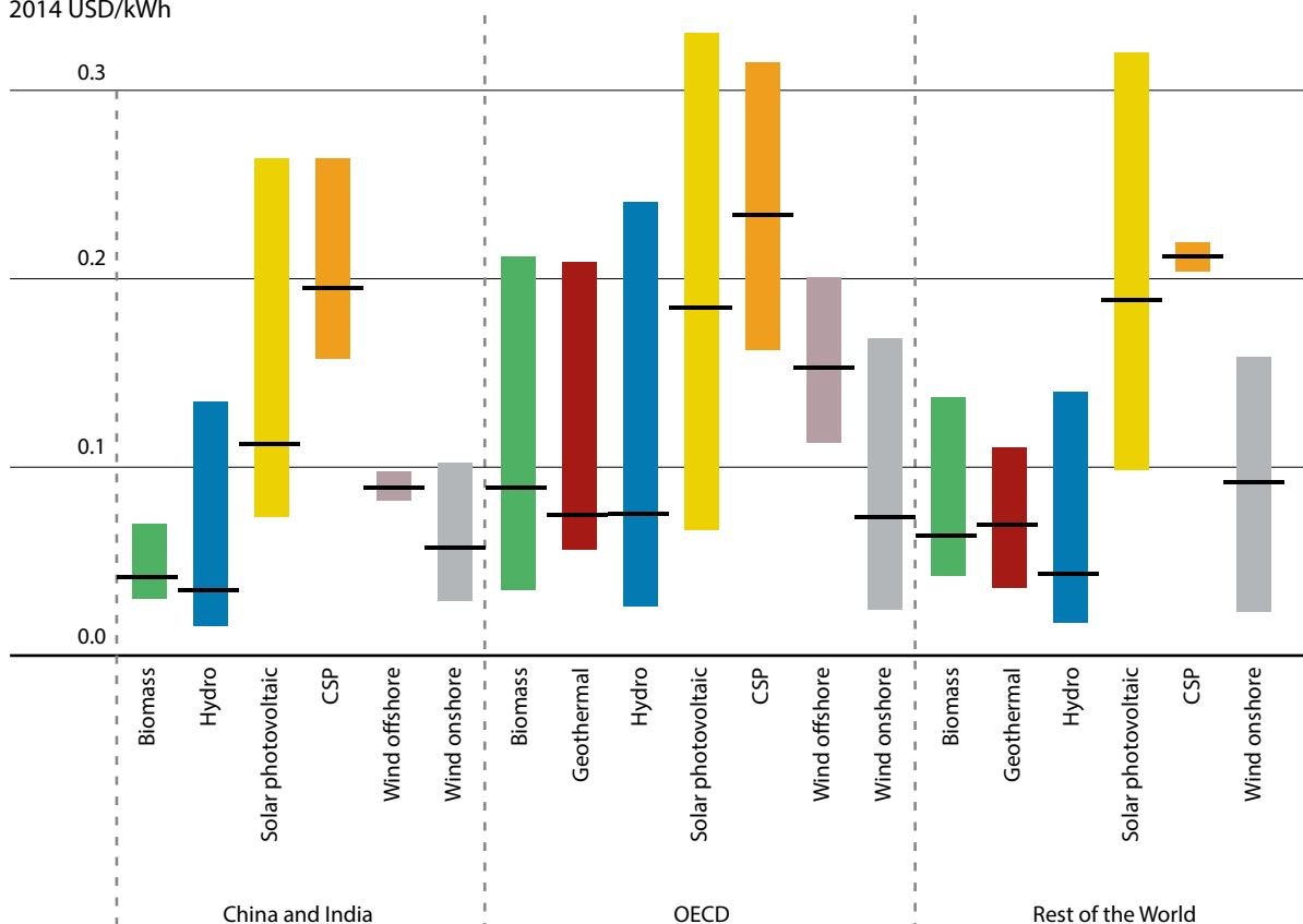
FIGURE 2.7: THE LEVELISED COST OF ELECTRICITY BY REGION AND TECHNOLOGY AND THEIR WEIGHTED AVERAGE, 2013/2014
