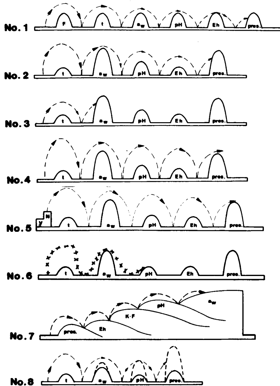
Fig. 1. Illustration of the hurdle effect, using eight examples. Symbols have the following meaning: F, heating; t, chilling; a_w , water activity; pH, acidification; E_h , redox potential; pres., preservatives; K-F, competitive flora; V, vitamins; N, nutrients.
